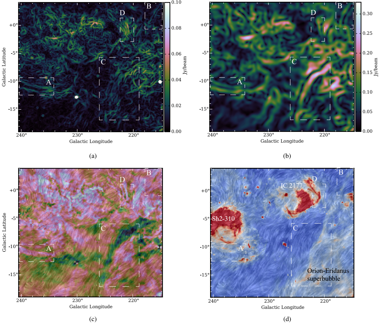
Figure 11. Anti-centre Galactic field including the HII region Sh2-310, the nebula IC 2177 and a part of the Orion-Eridanus superbubble. The panel (a) shows the |\nabla P| map at the original resolution, panel (b) shows the |\nabla P| map at \sim 136 arcmin, panel (c) shows the B -mode map overlaid with the magnetic field line direction in drapery texture and panel (d) shows the H\alpha overlaid with the same drapery texture. White dashed boxes indicate areas where |\nabla P| and B -mode features are correlated. No colour-bar is displayed on Figures (c) and (d) because the drapery structure alters the colour scale.
