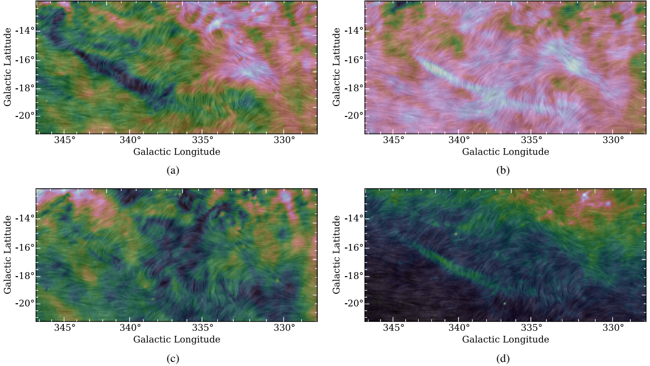
Figure 5. (a) and (b) show respectively the E - and B -mode maps, (c) shows the amplitude of the linear polarisation vector, |\mathbf{P}| , and (d) shows the H\alpha map. All maps are overlaid with the orientation of the magnetic field using the LIC technique. No colour-bar is displayed on these figures because the drapery structure alters the colour scale.
