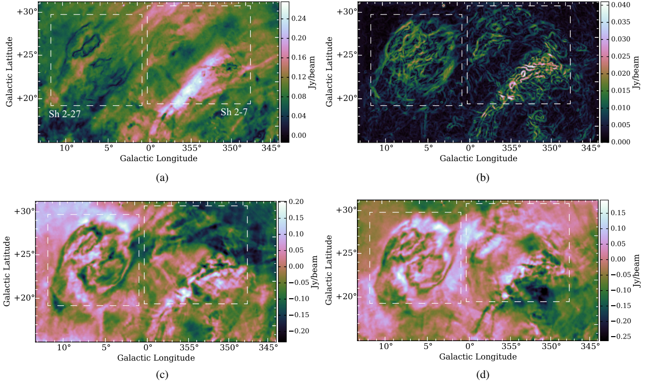
Figure 10. A subregion of the S-PASS survey including the HII regions Sh 2-7 and Sh 2-27. (a) shows the polarised intensity, (b) shows the |\nabla P| map at its original resolution, and the E - and B -mode maps associated with the same region are shown in (c) and (d).
