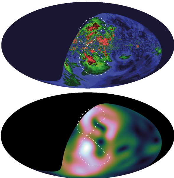
Figure 9. Top: Polarisation intensity of S-PASS data using the same colour scale and Aitoff projection as Carretti et al. (2013), Fig. 1. Bottom: |\nabla P| at scale of \sim 66^\circ on Aitoff projection. The dashed line delineate the giant radio lobes.
