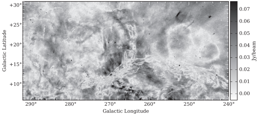
Figure 8. |P| of a subregion of the S-PASS data including the old SNRs Antlia (McCullough et al. 2002) (the hearth shape on the left hand side of the figure) and a part of the Gum Nebula (Purcell et al. 2015) (the arc at the bottom half on the right hand side of the figure) where many depolarisation canals are present.
